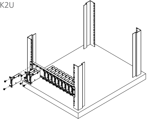
VE-RMK3U
