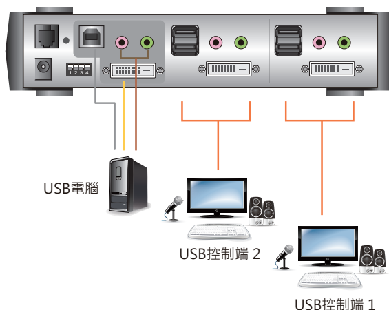
CS261 / CS261TK (背視圖)
