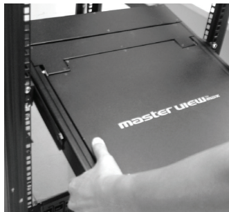
2. Slide the LCD KVM Switch / LCD Console onto the rails and secure it to the rack.
